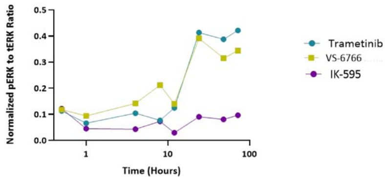
NCI-H2122: KRAS G12C Lung Tumor Model
