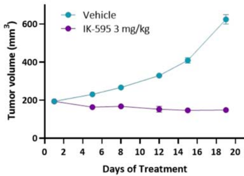
5637: CRAF Amplified Bladder Tumor Model
